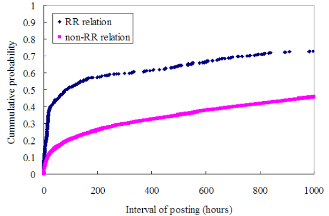
Fig. 10: Interval of posting between RR blogs (We have respectively investigated 699 and 9682 pairs of RR blogs and non-RR blogs)
