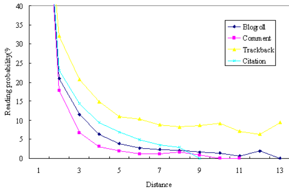
Fig. 7: Distance versus probability of reading relation (defined by browsing at least once)
