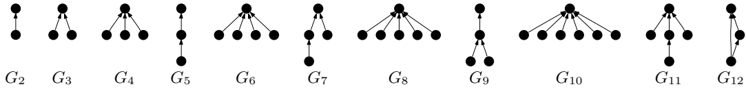
Fig. 2: Common cascade shapes, ordered by the frequency in the dataset
