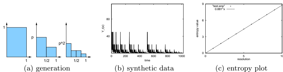
Fig. 6: Illustration of the b-model: (a) the recursive 80-20 procedure in its first three iterations (b) the generated synthetic activity (eg., number of posts, over time) (c) its entropy plot (entropy versus resolution - see text) Because the synthetic input traffic is self-similar, the entropy plot is linear, that is, scale free. Its slope is 0.881, much different than 1.0, which would be the uniform distribution (50-50)
