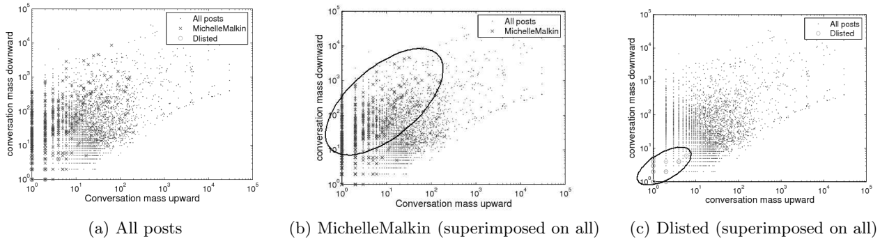
Fig. 4: Conversation mass for posts, an aspect of POSTFEATURES6. The top figure shows the Dlisted and MichelleMalkin clusters superimposed over points for all posts. The next two show the clusters separately, superimposed on all blog points for reference. Ovals are drawn around the main clusters. Note that while there is overlap between posts features of two blogs, they have different centers. This tells us that different blogs maintain different means and variances in conversation masses
